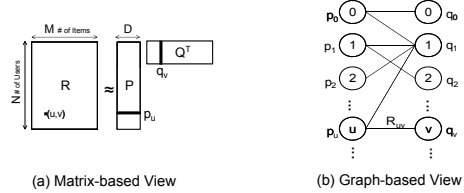
Figure 1: Collaborative Filtering.
