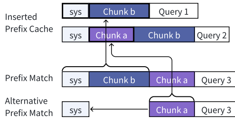
Fig. 10. Query 3 uses alternative path to match Chunk a .
