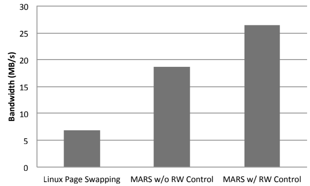
Fig. 9. The read bandwidth when page swapping
