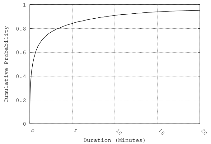
Fig. 1. Application usage for 12 Android users over 2 months We have developed an Android application, called “Astat”, to trace the application interleaving on Android phones. The application usage traces are collected by Astat installed on the smartphones with the permission of the volunteers. There are 25948 application interactions in the traces. The number of the durations less than 10 seconds is 10345. There are 16946 application interactions that last less than 1 minute. Many mobile applications last only a few seconds but used very frequently, such as messaging, weather report, and utility applications. For example, the application Wechat has 1624 interactions that are less than 10 seconds in the traces.
