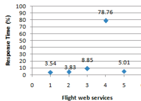
b). Comparisons of minimum results received in terms of response time of each flight booking WS
