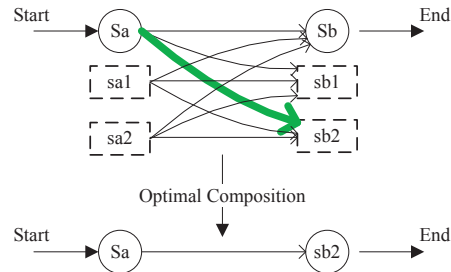
b.) Optimal composition of web services
